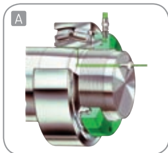
A HMV ..E nut for driving the bearing onto a tapered seating.
