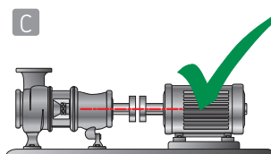
A Parallel misalignment (or offset) B Angular misalignment C Correct alignment
